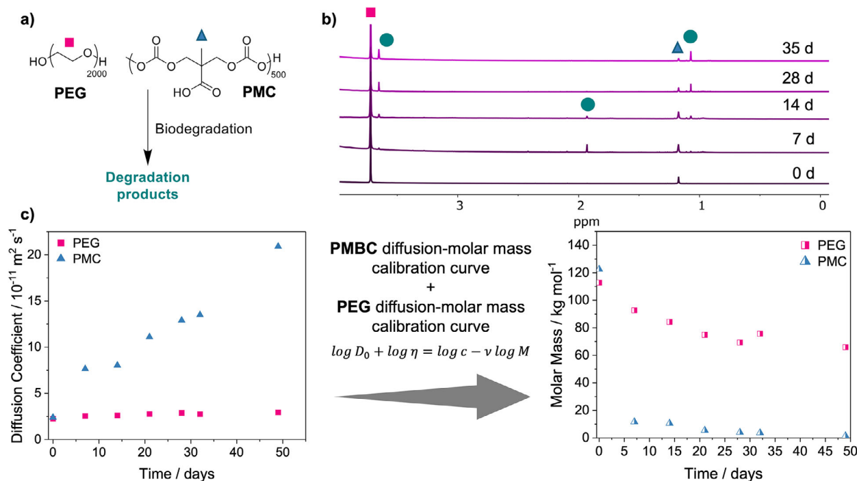
Figure 5. a) Scheme of biodegradation of PMC and PEG. b) Stacked ^1\text{H} NMR spectra (300 MHz, \text{H}_2\text{O} ) over time for biodegradation of PEG and PMC. c) Diffusion coefficients of PMC and PEG at infinite dilution over time being converted via PMBC calibration curve for PMC and PEG calibration curve for PEG polymers to molar mass over time.
